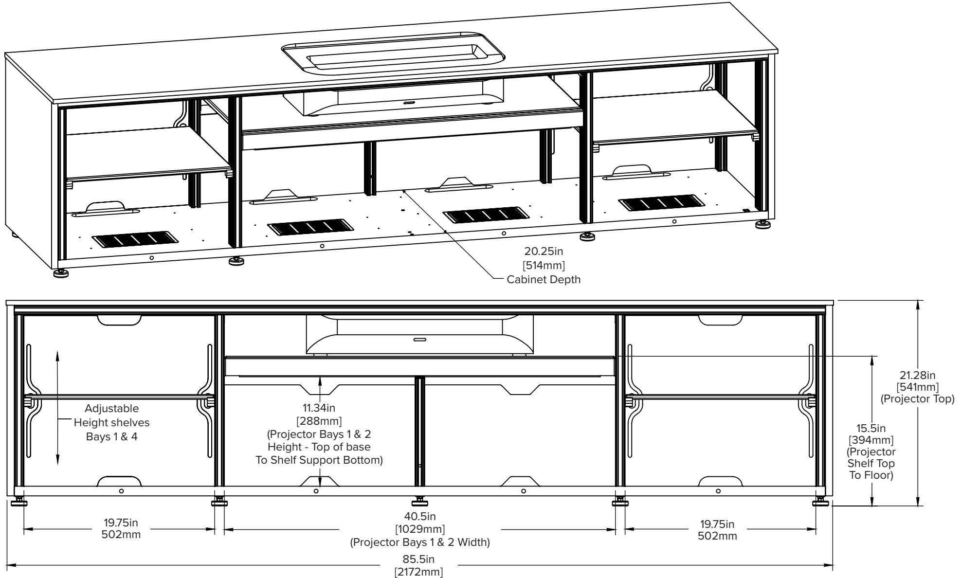
FRONT VIEW (Doors And Front Panel Removed For Clarity)
